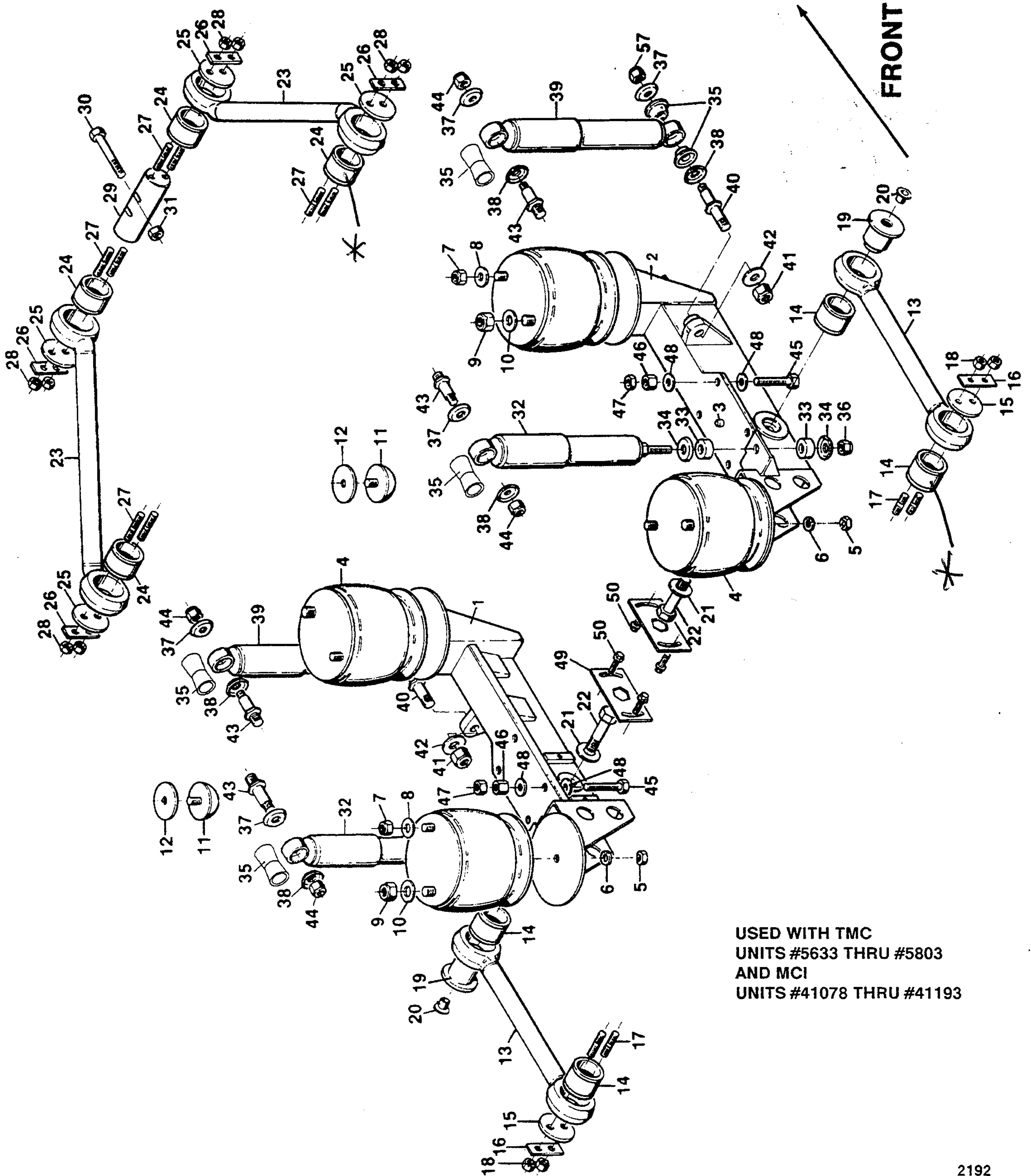
SUSPENSION ASSEMBLY - REAR DRIVE AXLE (USED PRIOR TO TMC UNIT #5803 & MCI UNIT #41193)
