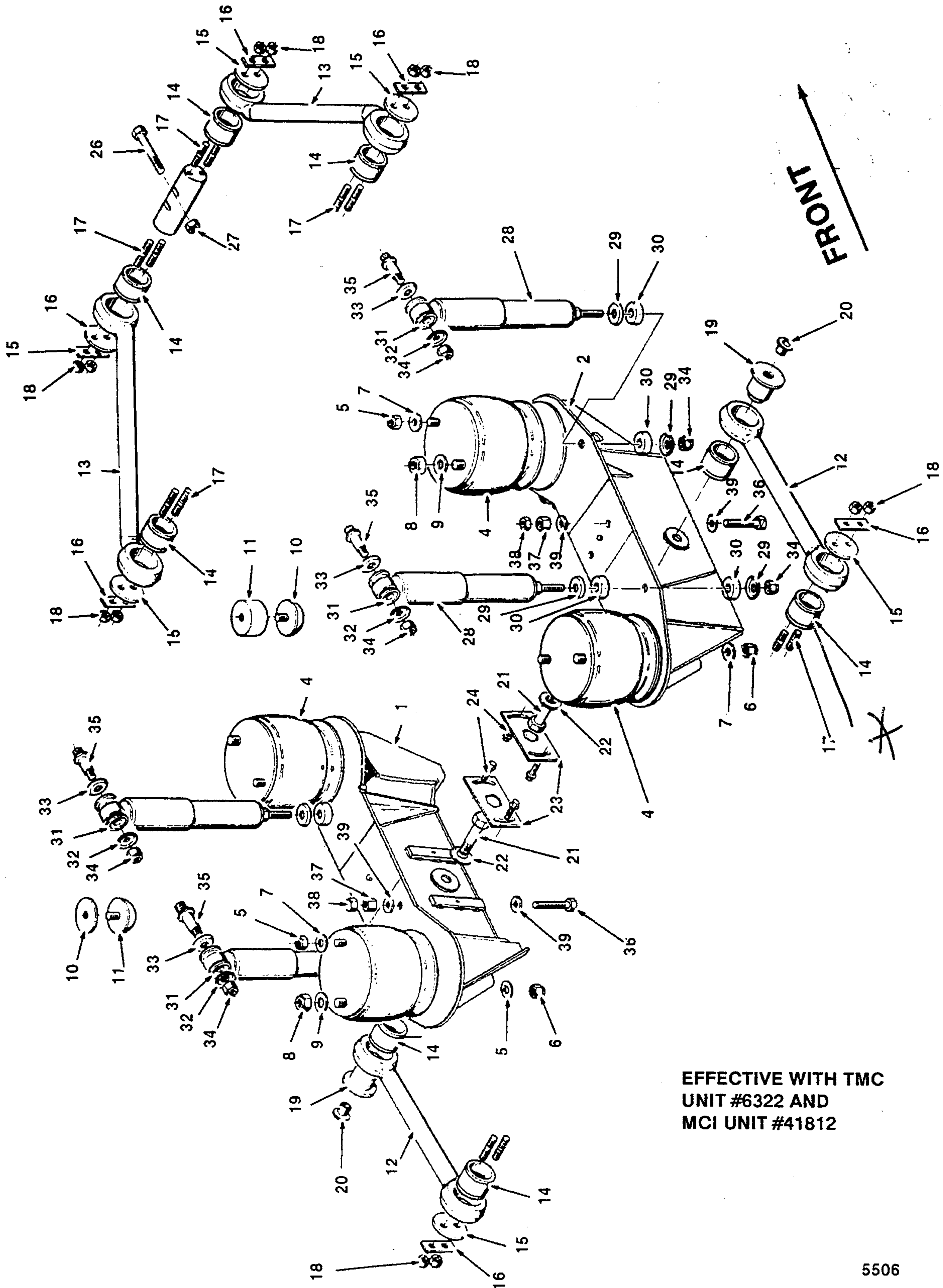
SUSPENSION ASSEMBLY - REAR DRIVE AXLE (EFFECTIVE WITH TMC UNIT #6322 & MCI UNIT #41812)
